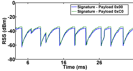
Fig. 10. RSS signatures measured by ZigBee when LoRa transmits 0x00, and 0xC0, respectively.
