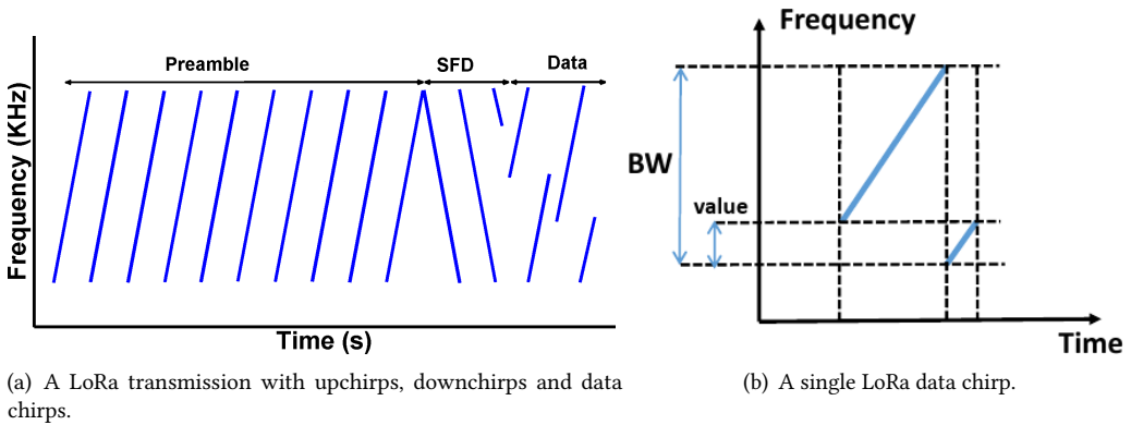
Fig. 2. LoRa modulation.
