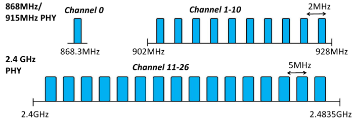
Fig. 3. IEEE 802.15.4 channels.
