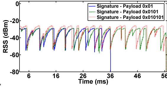
Fig. 9. RSS signatures measured by ZigBee when LoRa transmits 0x01, 0x0101, and 0x010101, respectively.
