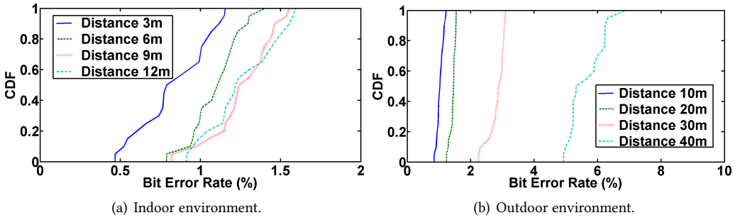
Fig. 21. BER measurements in indoor and outdoor environments.
